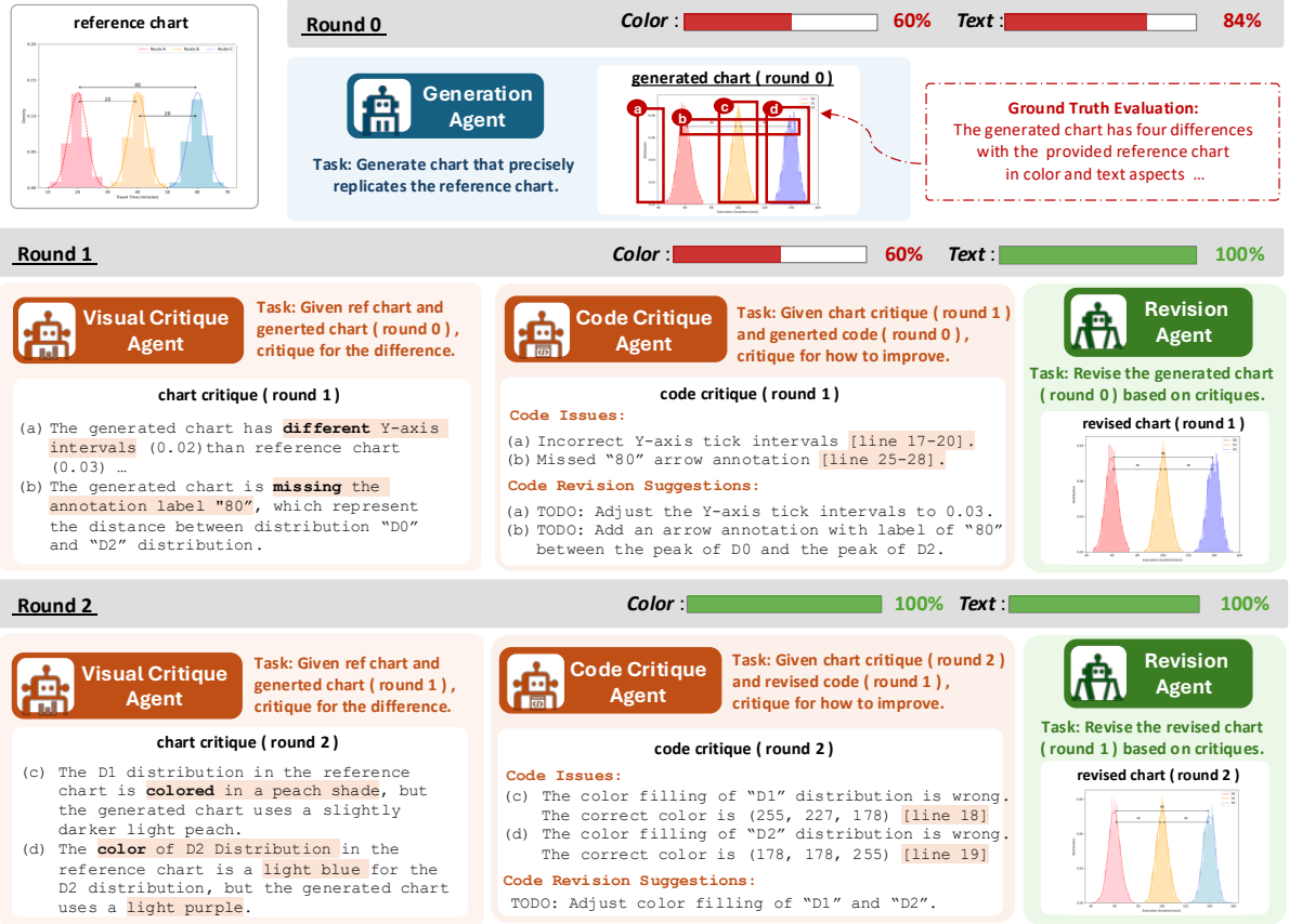
Figure 5: Case study of METAL’s progressive refinement from initial generation to perfect accuracy. Starting from Round 0’s initial generation (60% color accuracy, 84% text accuracy), the system iteratively improves the output. In Round 1, the system identifies and corrects Y-axis scale issues and missing annotations, achieving 100% text accuracy. Round 2 refines the color representations of distributions, achieving perfect accuracy across all metrics.
